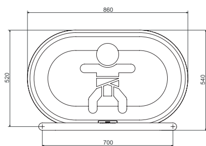
Installation Dimensions in mm
