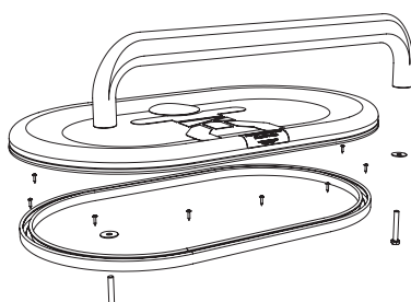
Exploded view of fixing method
